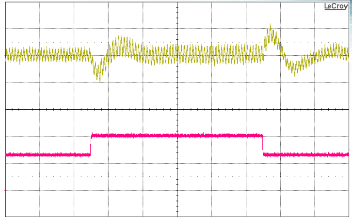
Figure 8: Output voltage response to step-change in load current with 200µF hold-up capacitor (50%-75%-50% of Iout(max), 115Vrms, 60Hz) Top: Vout (1V/div), Bottom: Iout (5A/div), Timebase: (100ms/div).
